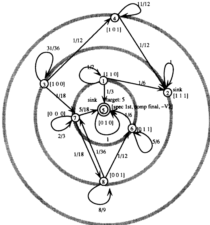
Fig. 1. The eight parameter settings in the GW example, shown as a Markov structure. Directed arrows between circles (states, parameter settings, grammars) represent possible non-zero (possible learner) transitions. The target grammar (in this case, number 5, setting [0 1 0]), lies at dead center. Around it are the three settings that differ from the target by exactly one binary digit; surrounding those are the three hypotheses two binary digits away from the target; the third ring out contains the single hypothesis that differs from the target by three binary digits. Note that the learner can either stay in the same state or step in or out one ring (binary digit) at a time, according to the single-step learning hypothesis; but some transitions are not possible because there is no data to drive the learner from one state to the other under the TLA. Numbers on the arcs denote transition probabilities between grammar states; these values are not computed by the original GW algorithm. The next section shows how to compute these values, essentially by taking language set intersections.
